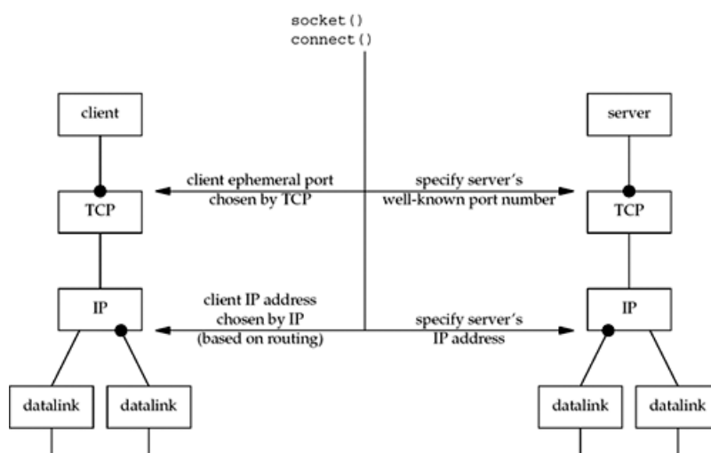
Figure 5.15. Summary of TCP client/server from client's perspective.
