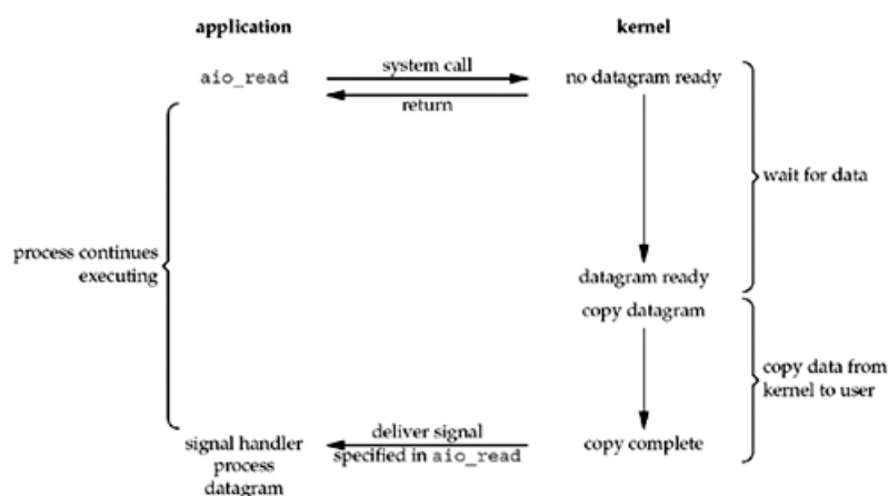
Figure 6.5. Asynchronous I/O model.
