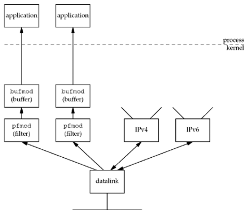
Figure 29.2. Packet capture using DLPI, pfmod , and bufmod .
