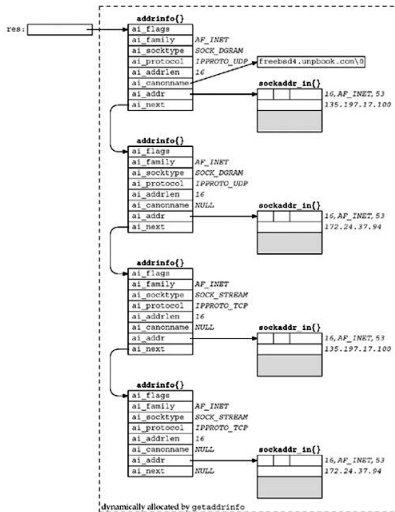
Figure 11.5. Example of information returned by getaddrinfo .
