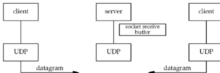
Figure 8.6. Summary of UDP client/server with two clients.
