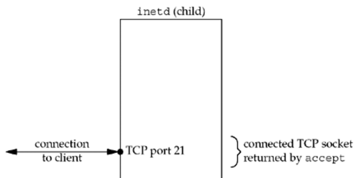
Figure 13.9. inetd descriptors in child.
