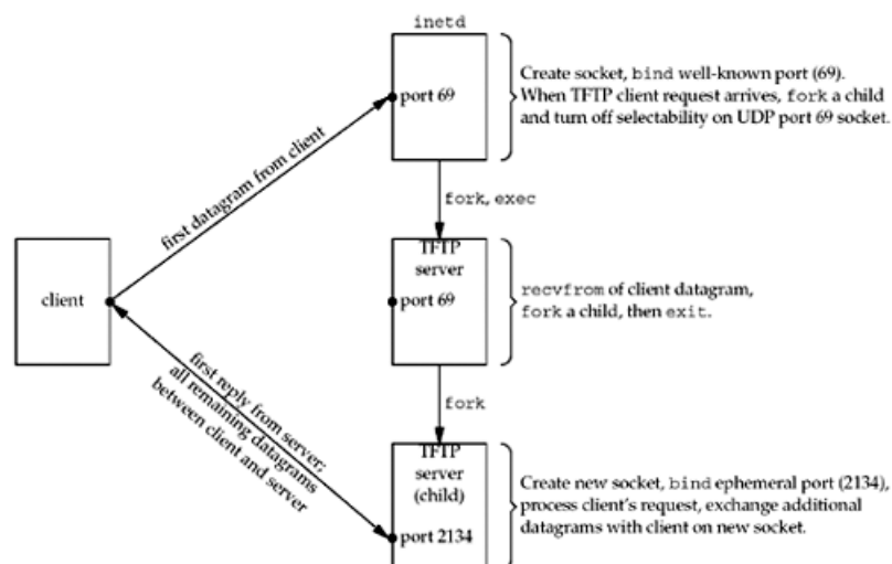
Figure 22.20. UDP concurrent server invoked by inetd .
