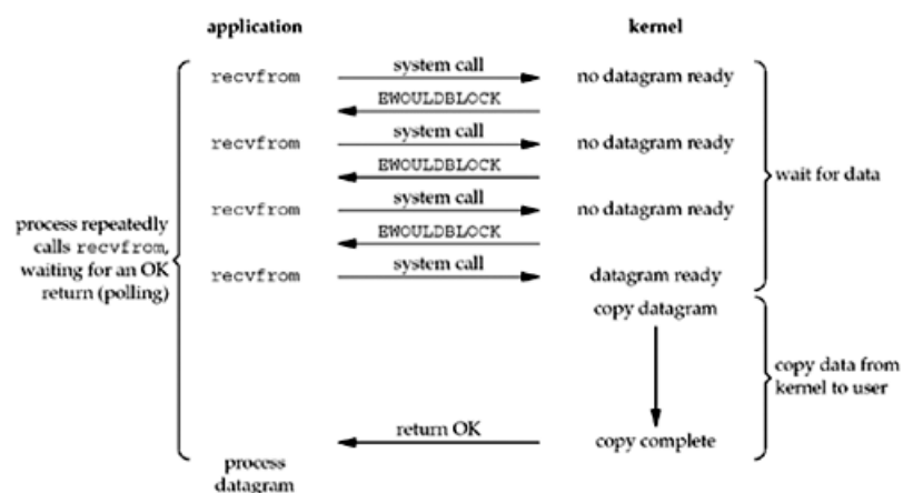
Figure 6.2. Nonblocking I/O model.
