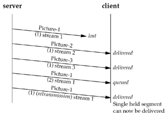
Figure 10.6. Sending three pictures over three SCTP streams.
