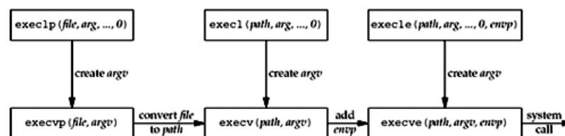
Figure 4.12. Relationship among the six exec functions.
