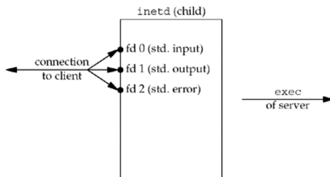
Figure 13.10. inetd descriptors after dup2 .
