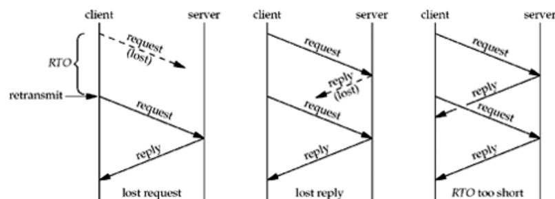
Figure 22.5. Three scenarios when retransmission timer expires.
