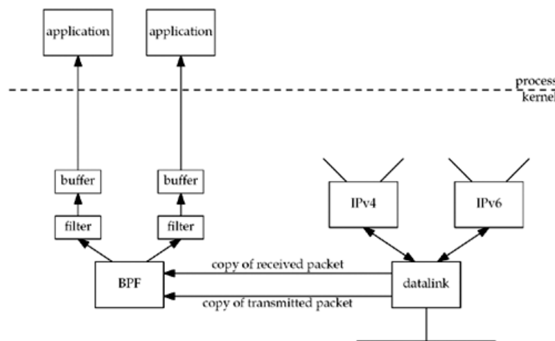
Figure 29.1. Packet capture using BPF.
