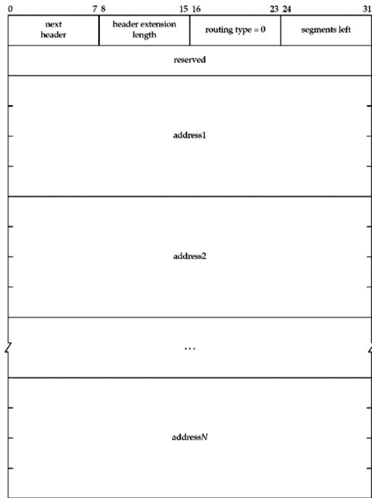
Figure 27.11. IPv6 routing header.
