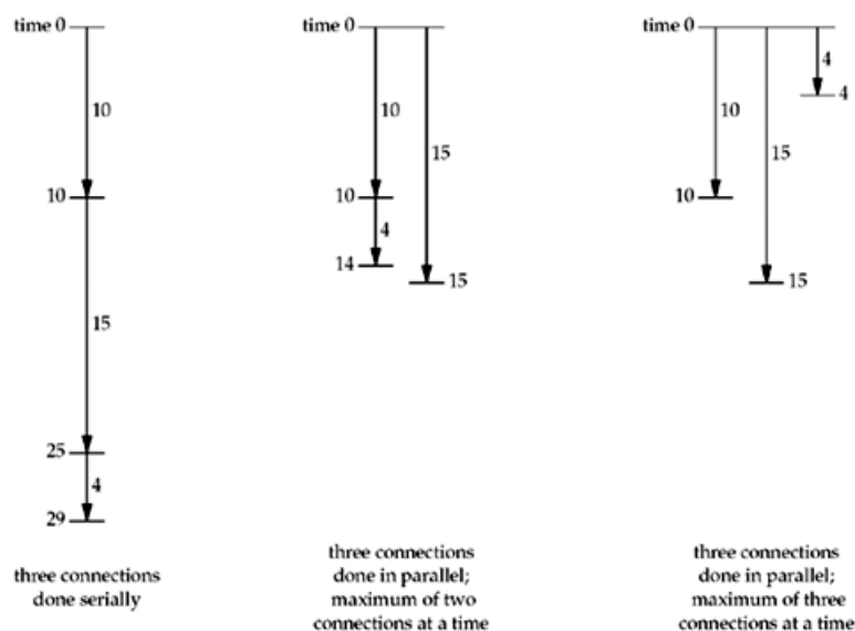
Figure 16.12. Establishing multiple connections in parallel.
