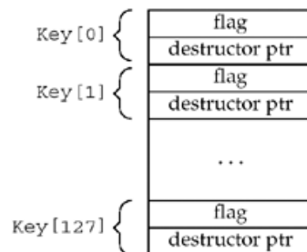
Figure 26.7. Possible implementation of thread-specific data.
