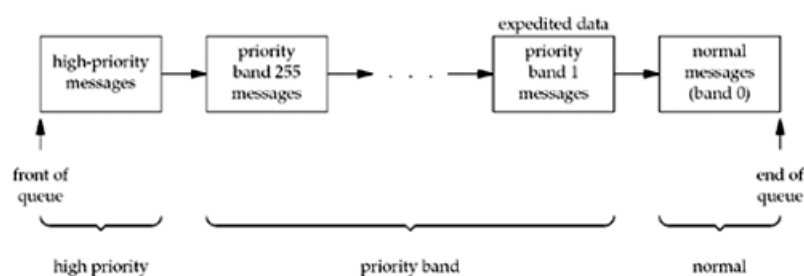
Figure 31.5. Ordering of STREAMS messages on a queue, based on priority.
