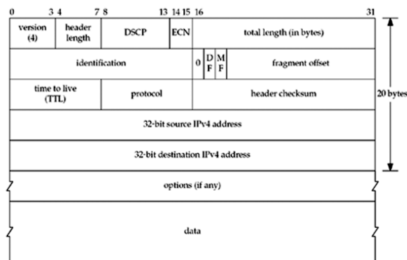
Figure A.1. Format of the IPv4 header.
