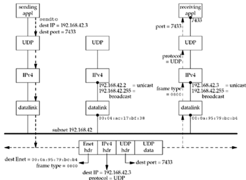
Figure 20.3. Unicast example of a UDP datagram.
