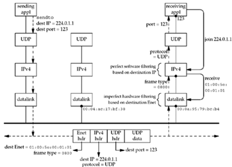
Figure 21.4. Multicast example of a UDP datagram.
