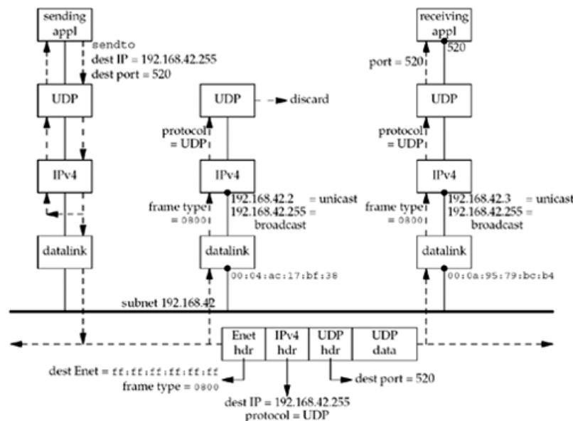
Figure 20.4. Example of a broadcast UDP datagram.
