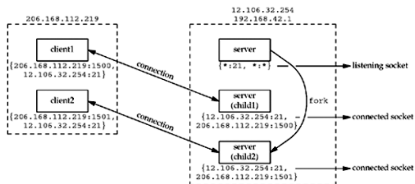
Figure 2.14. Second client connection with same server.
