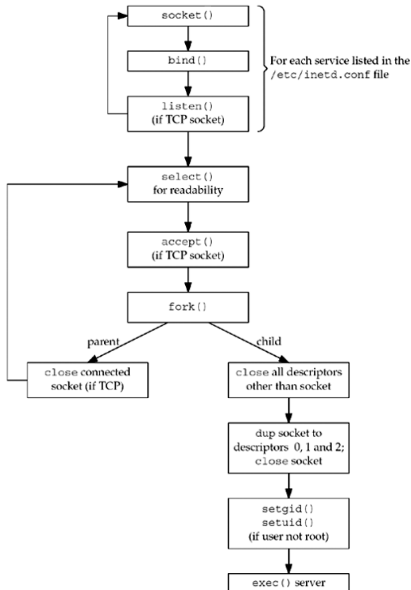
Figure 13.7. Steps performed by inetd .
