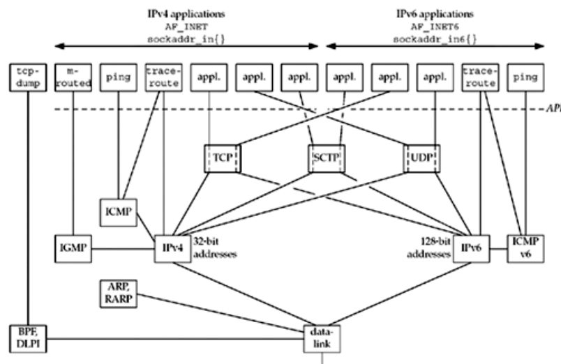
Figure 2.1. Overview of TCP/IP protocols.
