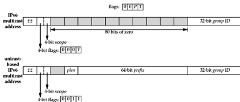
Figure 21.2. Format of IPv6 multicast addresses
