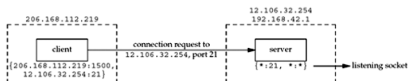
Figure 2.12. Connection request from client to server.
