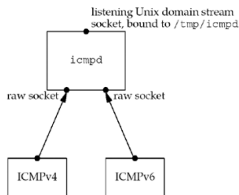
Figure 28.26. icmpd daemon: initial sockets created.
