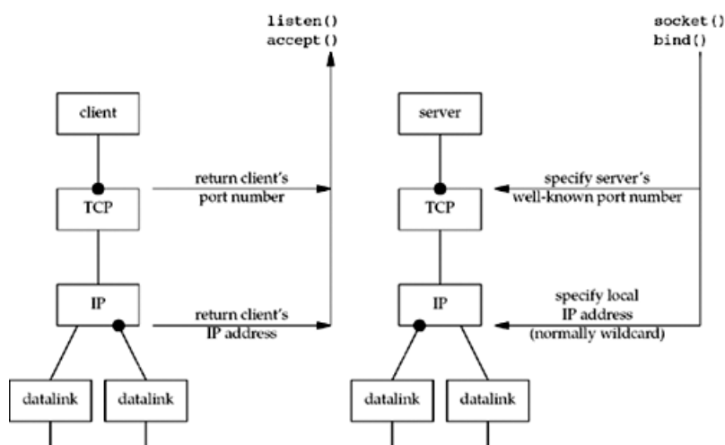
Figure 5.16. Summary of TCP client/server from server's perspective.
