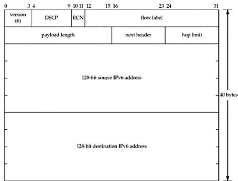
Figure A.2. Format of the IPv6 header.
