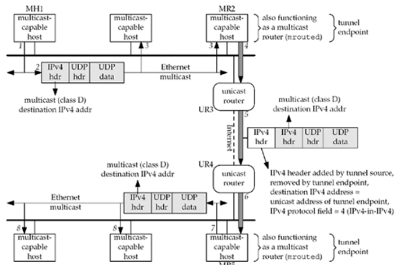
Figure B.1. IPv4-in-IPv4 encapsulation used on MBone.
