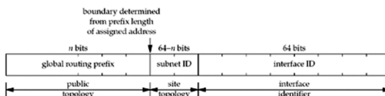
Figure A.8. IPv6 aggregatable global unicast addresses.
