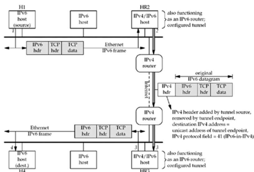
Figure B.2. IPv6-in-IPv4 encapsulation on 6bone.
