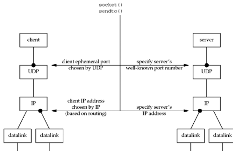
Figure 8.11. Summary of UDP client/server from client's perspective.
