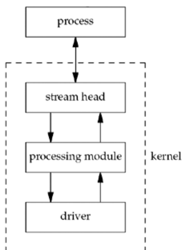
Figure 31.2. A stream with a processing module.
