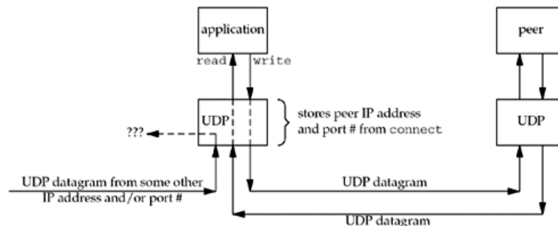
Figure 8.15. Connected UDP socket.
