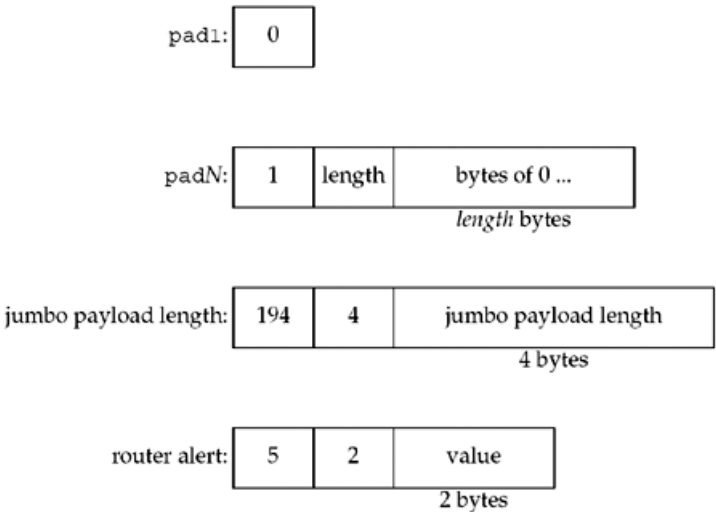
Figure 27.9. IPv6 hop-by-hop options.
