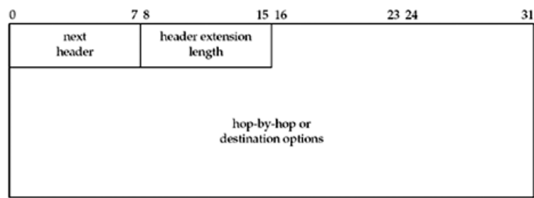
Figure 27.7. Format of hop-by-hop and destination options.
