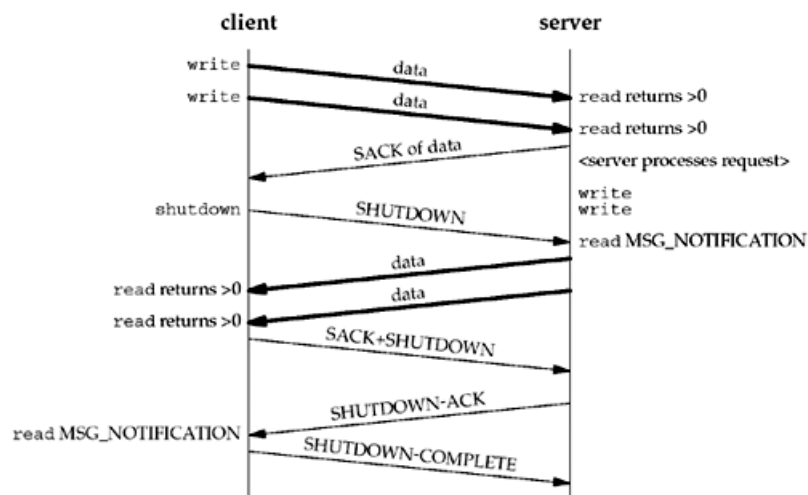
Figure 9.5. Calling shutdown to close an SCTP association.
