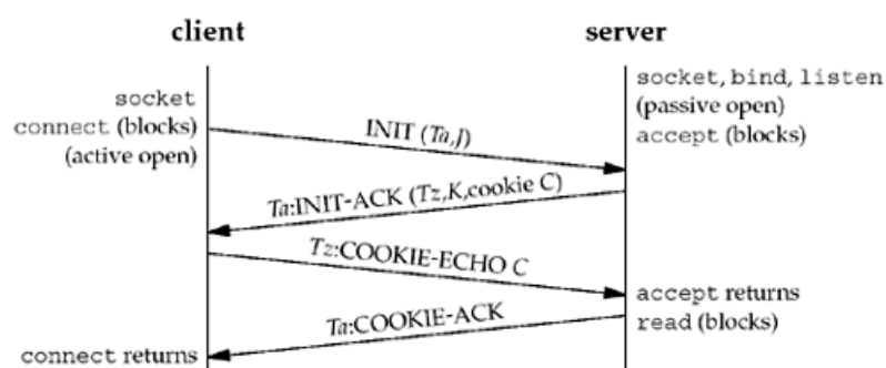
Figure 2.6. SCTP four-way handshake.
