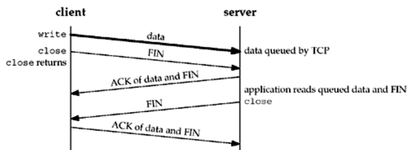
Figure 7.7. Default operation of close : it returns immediately.
