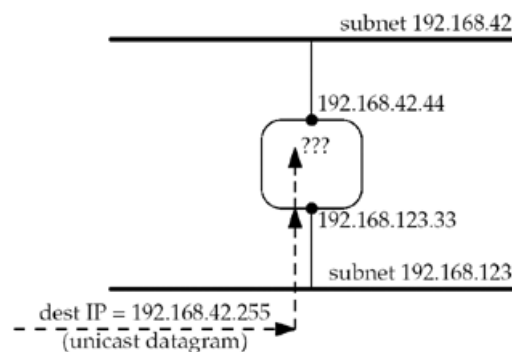
Figure 20.2. Does a router forward a subnet-directed broadcast?
